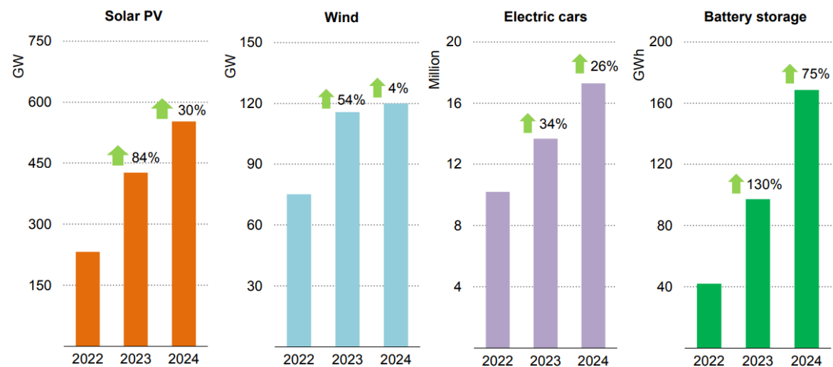
Annual capacity additions for selected energy technologies
