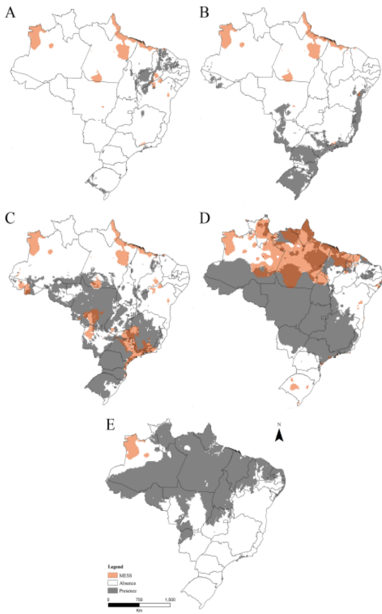
Fig 2. Potential distribution of the five species. (A) Potential distribution of Lampropeltis getula . (B) Potential distribution of Pantherophis guttatus . (C) Potential distribution of Lampropeltis triangulum . (D) Potential distribution of Python bivittatus . (E) Potential distribution of Python regius . Orange areas represent MESS regions with non-analogue climate.
