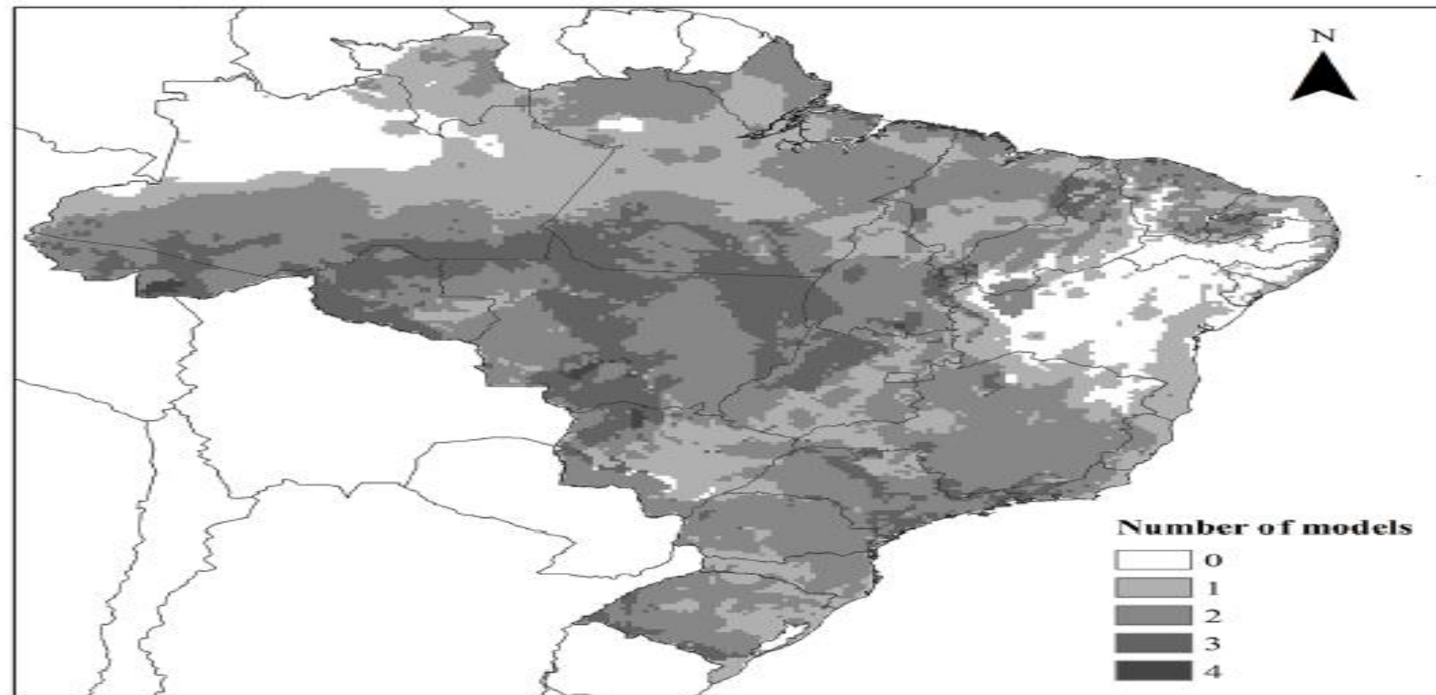
Fig 3. Consensus model of the potential distribution of the five species.
